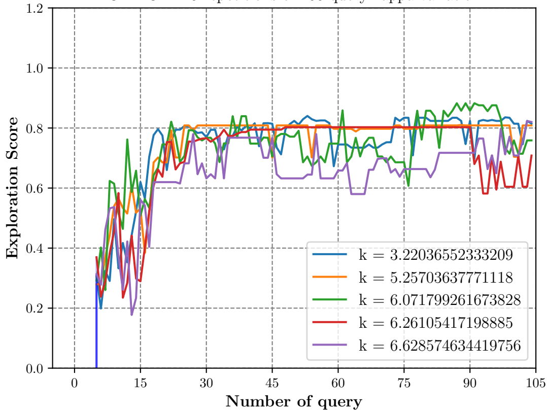
GP-BO_2D 5 repetitions of 100 query kappa variation
